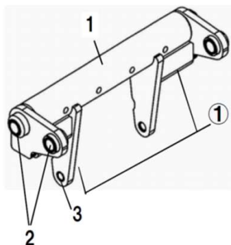
Drawing No. 3-9 Wheel Fork Assy
