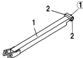
Drawing No. 3-13 Bogie Wheel Assy
