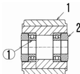
Drawing No. 3-11 Bogie Wheel Assy
