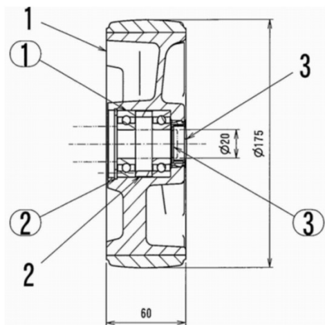
Drawing No. 4-3 Steering Wheel Assy
