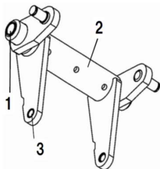
Drawing No. 3-7 Wheel Fork Assy
