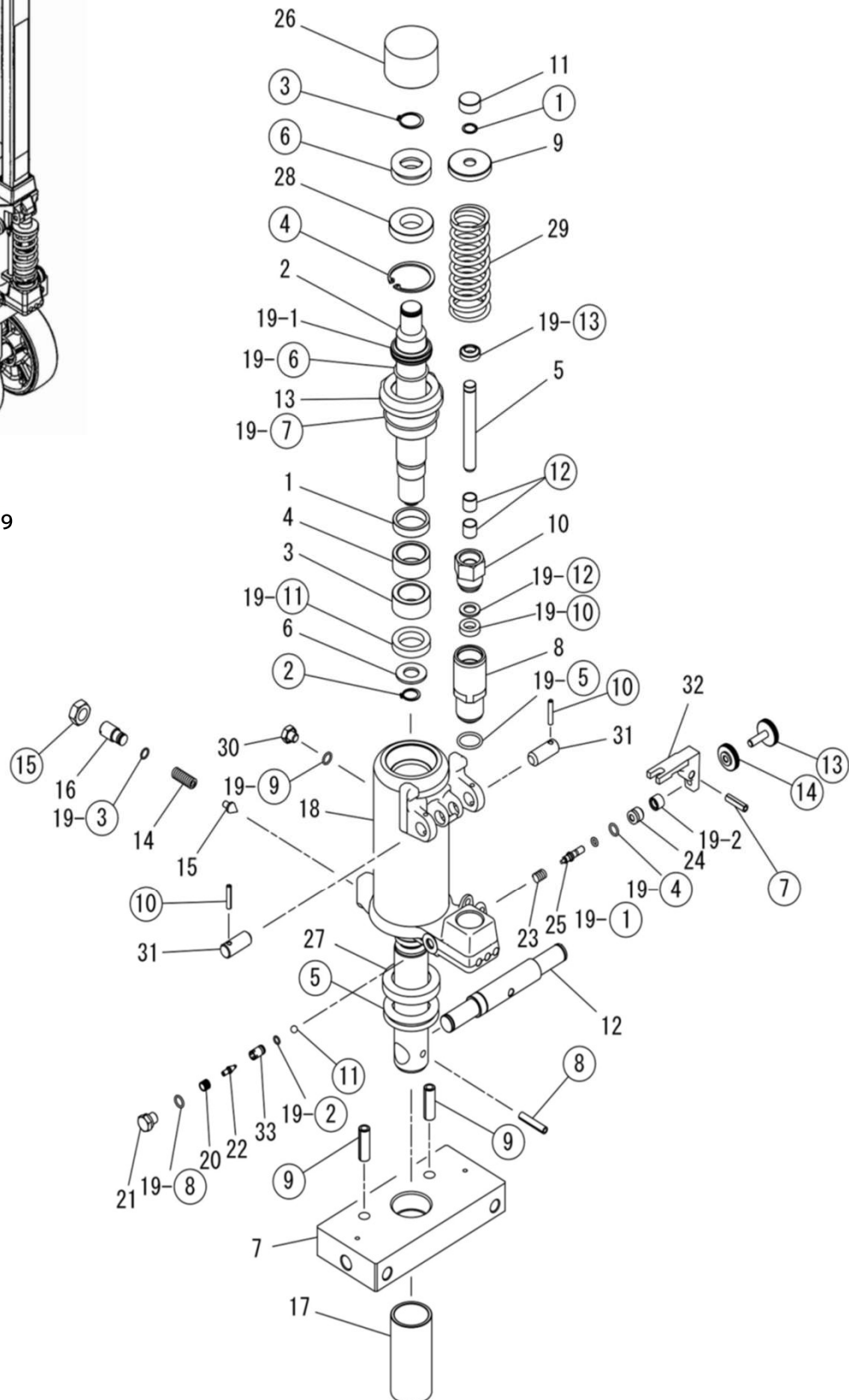
Drawing No. 4-1 Pump Unit Assy Drawing No. 4-1-19 Pump Unit Seal Kit
