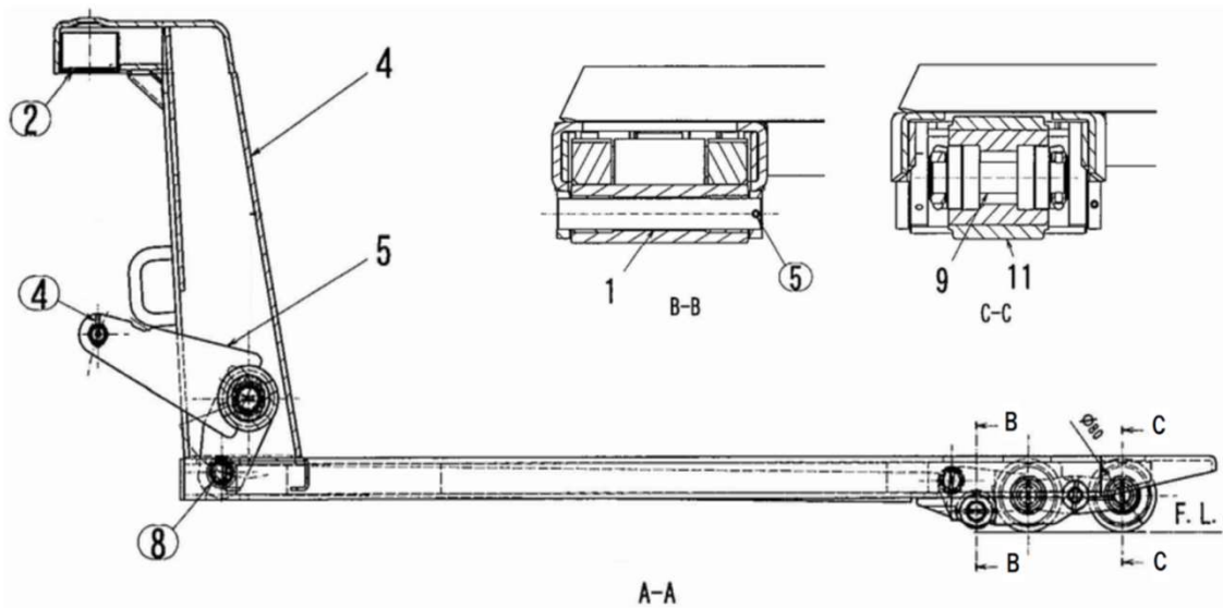
Drawing No. 3-5 Torsion Tube Assy
