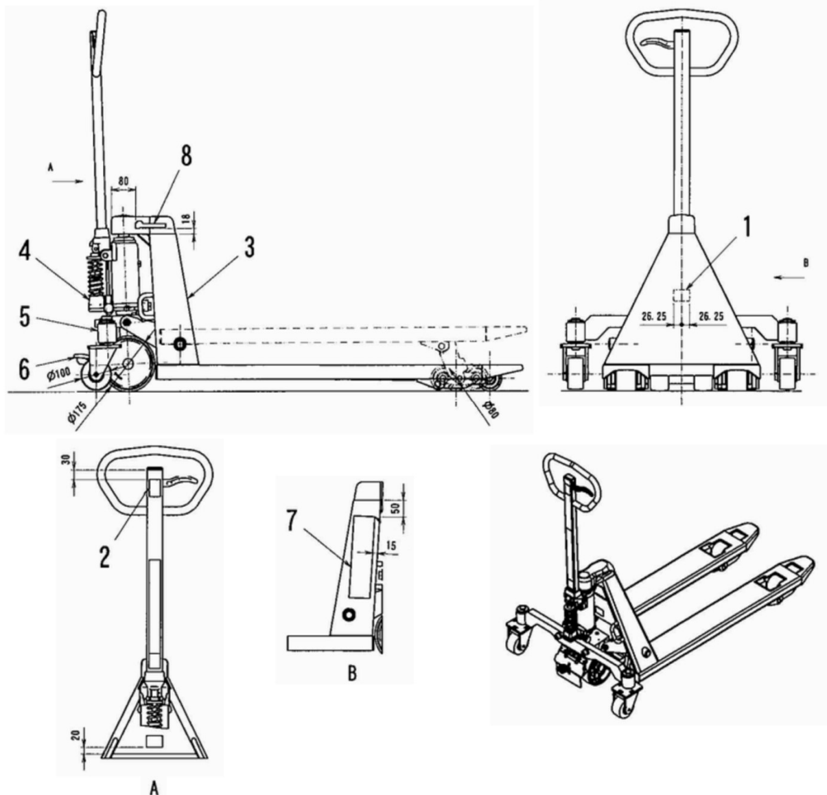
Drawing No. 1 - Name Plate
