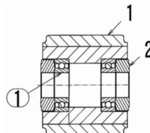
Drawing No. 3-13 Bogie Wheel Assy
