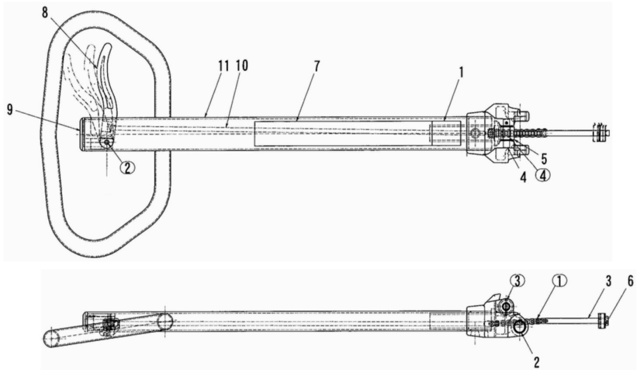
Drawing No. 4-2 Steel Handle Assy
